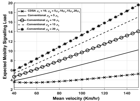
Fig. 14. Normalized expected signalling load vs mean velocity for c = 0.6 and E[\lambda] = 5 mins at high speeds
