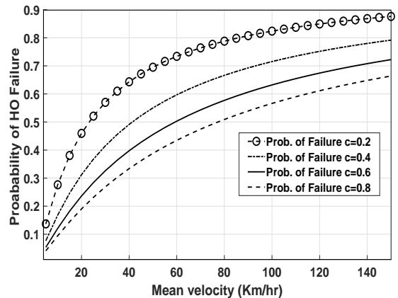
Fig. 9. Probability of HO failure vs mean velocity for different values of coverage factor. E[\lambda] = 5 mins and E[\rho] = 10
