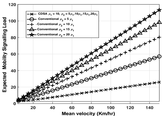
Fig. 13. Normalized expected signalling load vs mean velocity for c = 0.1 and E[\lambda] = 5 mins
