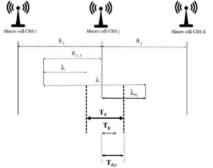
Fig. 3. Timing diagram of handover model parameters
