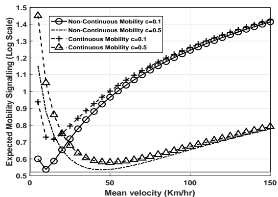
Fig. 15. Expected Mobility Signalling vs mean velocity in case of normal and continuous mobility for c = 0.1 and c = 0.5
