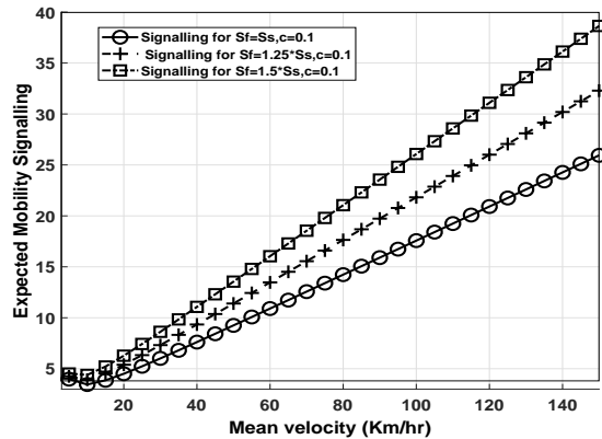
Fig. 16. Expected mobility signalling comparison of handover failure and success for c = 0.1 . E[\rho] = 10 indicating how handover failure results in more mobility signalling
