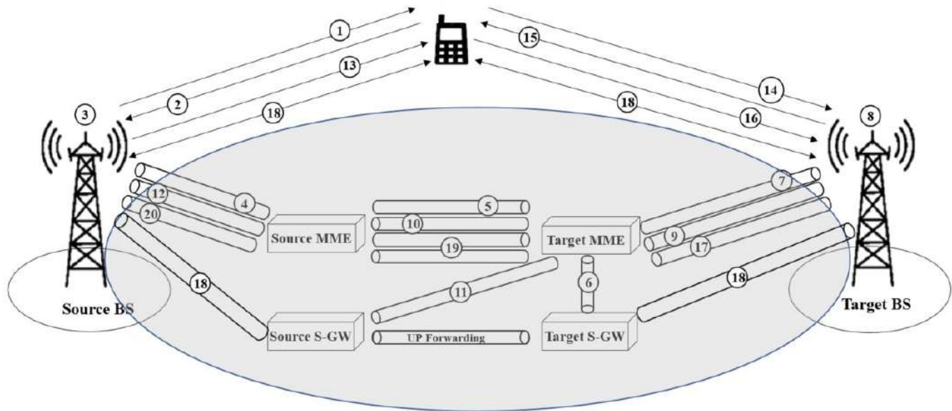
Fig. 1. Signalling messages exchanged with in a typical S1 handover scenario
