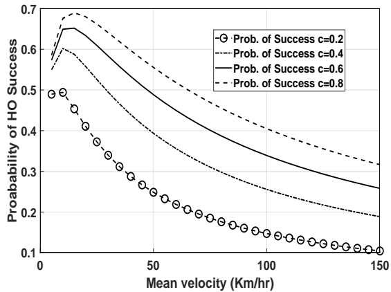
Fig. 10. Probability of HO success vs mean velocity for different values of coverage factor. E[\lambda] = 5 mins and E[\rho] = 10
