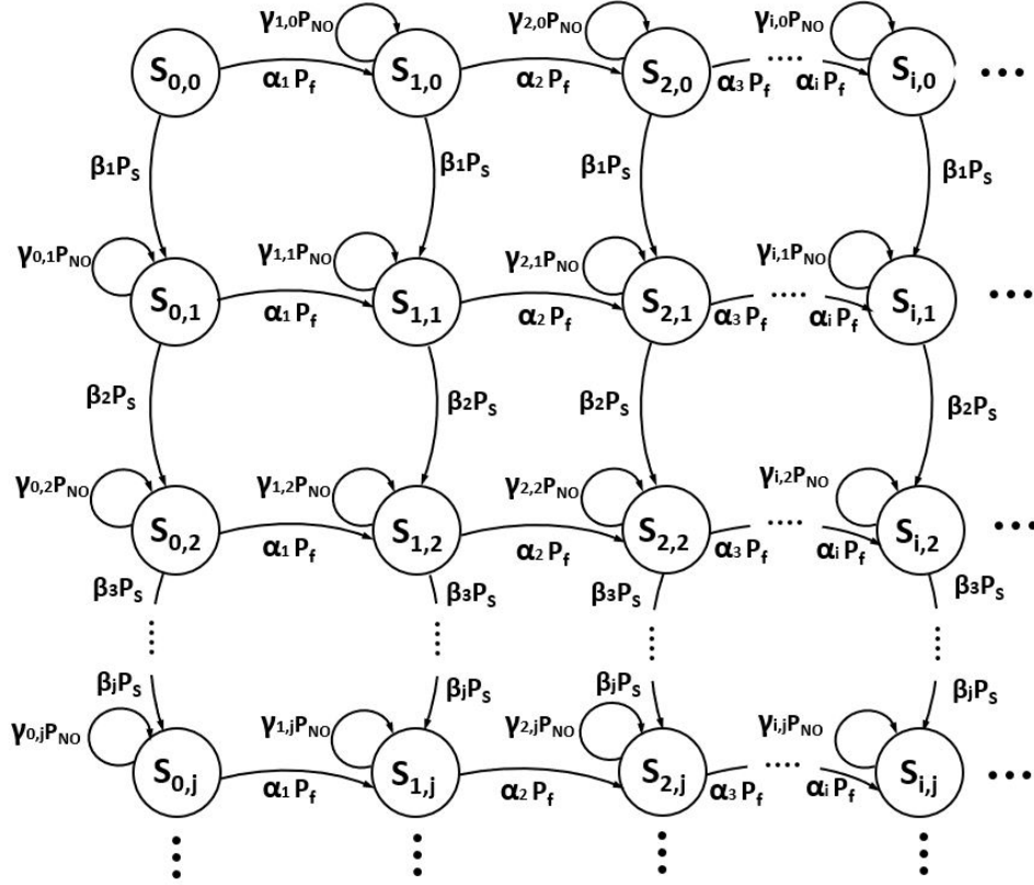
Fig. 5. Markov chain modeling of no-handover, handover failure and handover success related core-network mobility signaling
