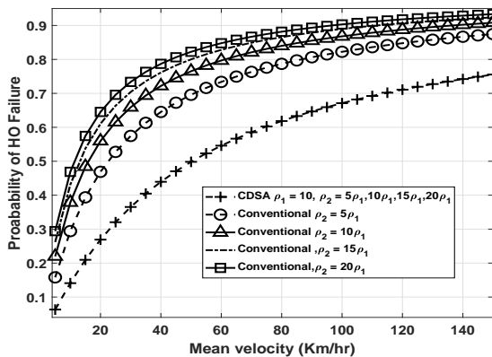
Fig. 11. Probability of HO failure vs mean velocity for different values of cell density. E[\lambda] = 5 mins and c = 0.5
