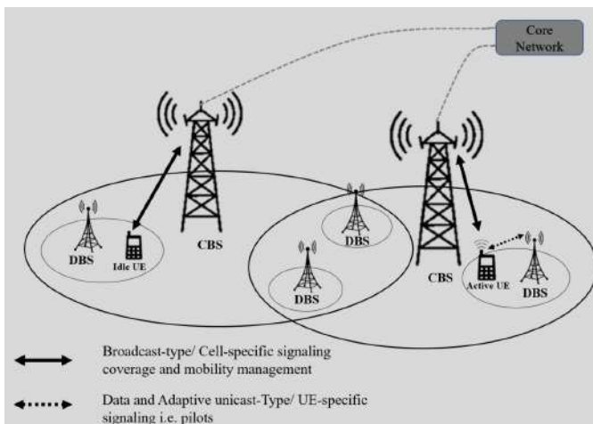
Fig. 2. Schematic of control data plane separated Architecture
