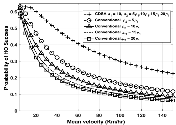
Fig. 12. Probability of HO success vs mean velocity for different values of cell density. E[\lambda] = 5 mins and c = 0.5
