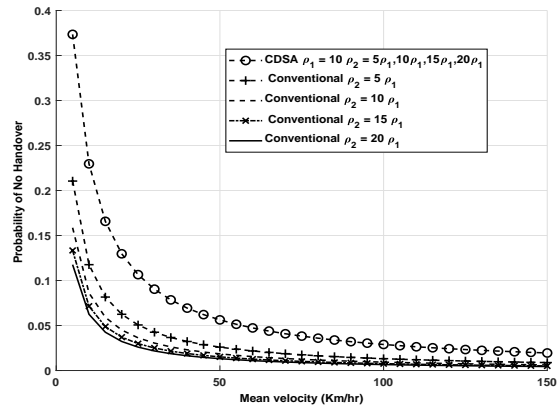
Fig. 8. Probability of no handover signalling vs mean velocity for CDSA and different cell densities of conventional network with E[\lambda] = 5 mins
