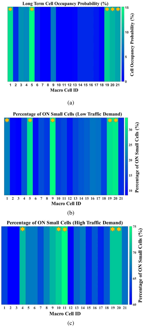
Fig. 12. (a) Long term Cell Occupancy probability (b) Percentage of ON Small Cells at Low Traffic Demand (c) Percentage of ON Small Cells at High Traffic Demand.
