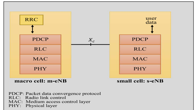
Fig. 10. Protocol stack of macro and small cells in dual connectivity with control-data separation [112].
