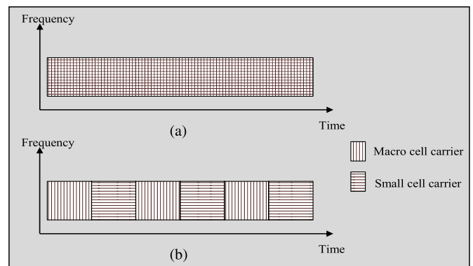
Fig. 11. Transmission/Reception modes for dual connectivity. (a) Simultaneous mode. (b) TDM mode.
