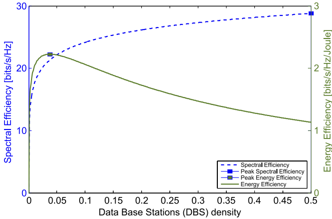
Fig. 3. Energy and spectral efficiencies vs DBS density [46].
