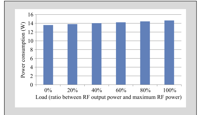
Fig. 2. Typical power consumption of pico BS in LTE system with 10 MHz bandwidth and 2 \times 2 MIMO configuration, based on the EARTH power model [25].
